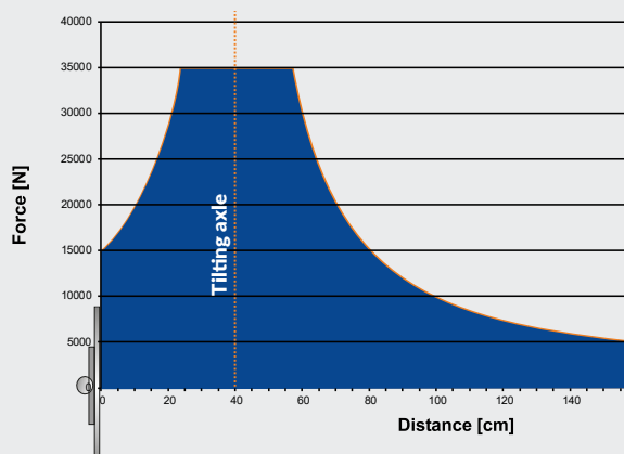
Max tilting torque 6000 Nm
