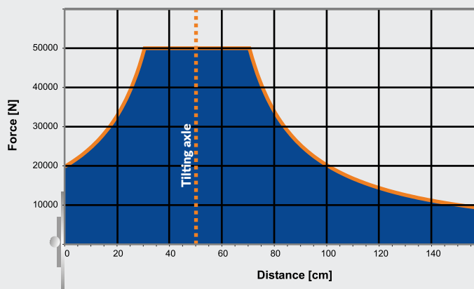
Distance from table plate to centre of gravity
