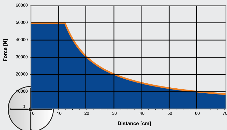
Distance from centre of table plate to centre of gravity
