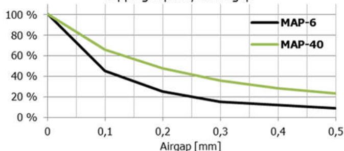
Gripping capacity vs. airgap
