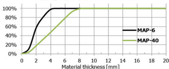
Gripping capacity vs. material thickness
